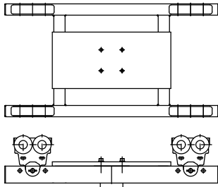
4-TROLLEY CARRIAGE
